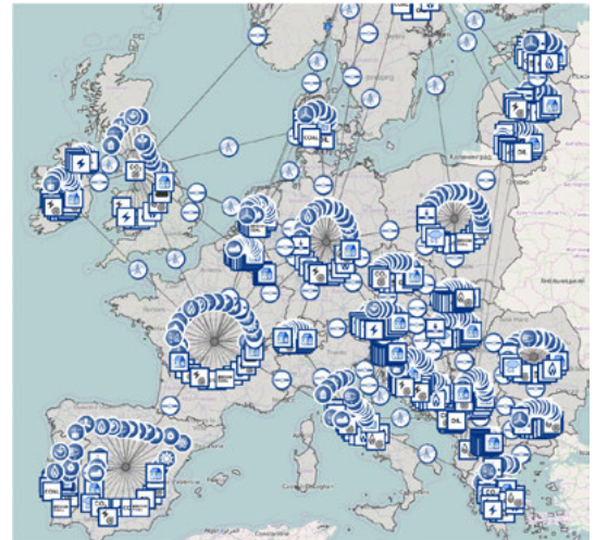
Figure 8: Power model
