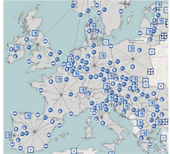
Figure 7: Gas model
