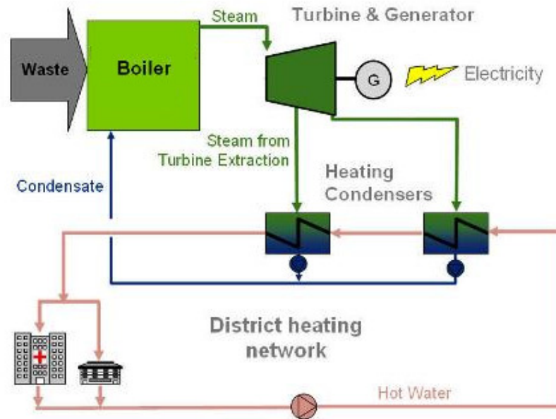
Figure 11: Illustration of district heating boiler, gas-fired (ref. /28/)
