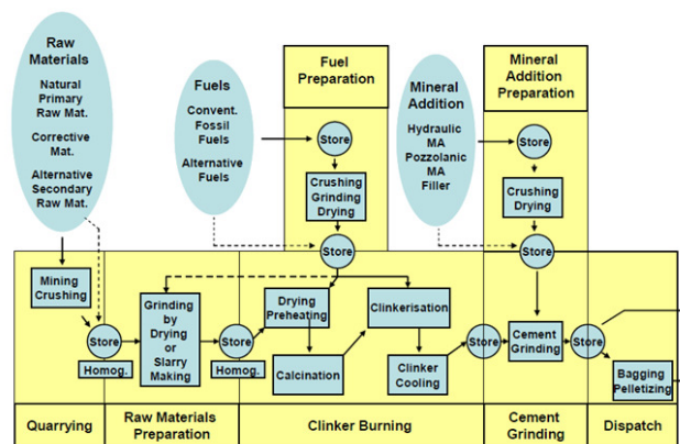
Figure 16: Simplified cement production process (ref. /22/)
