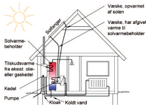
Figure 19: Illustration of a solar thermal heating system 5
