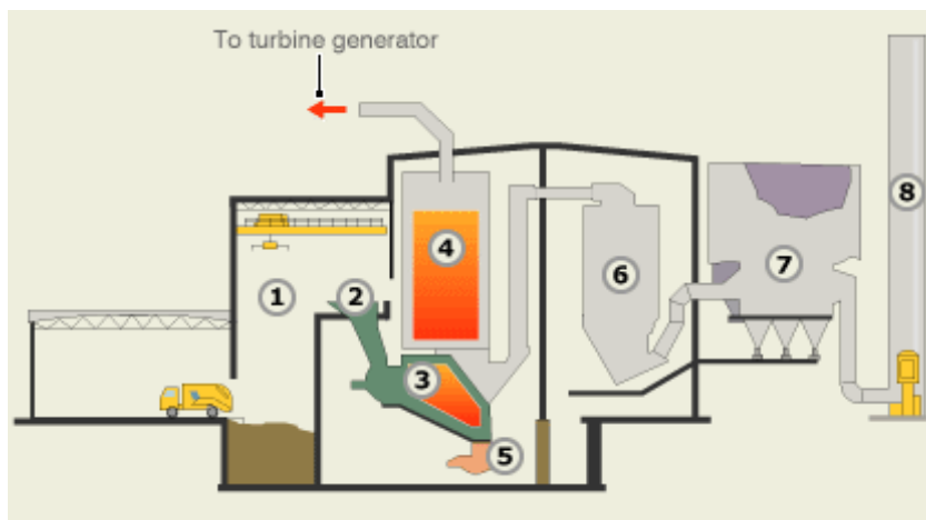
Figure 9: Illustration of an incineration plant (ref. /26/) 3
