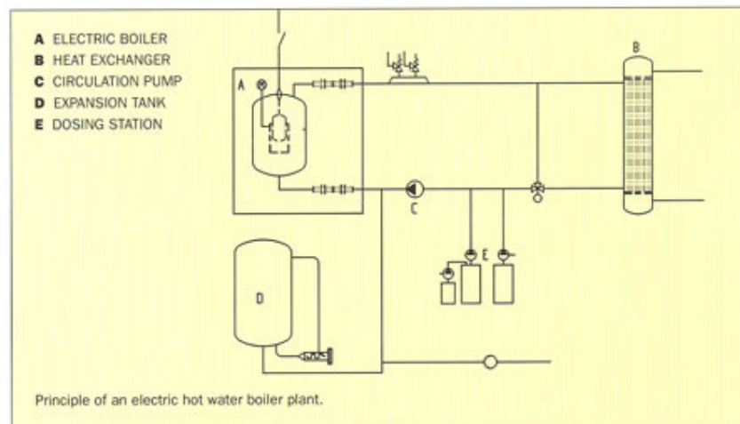
Figure 6: Illustration of a hot water boiler (reg. /24/)
