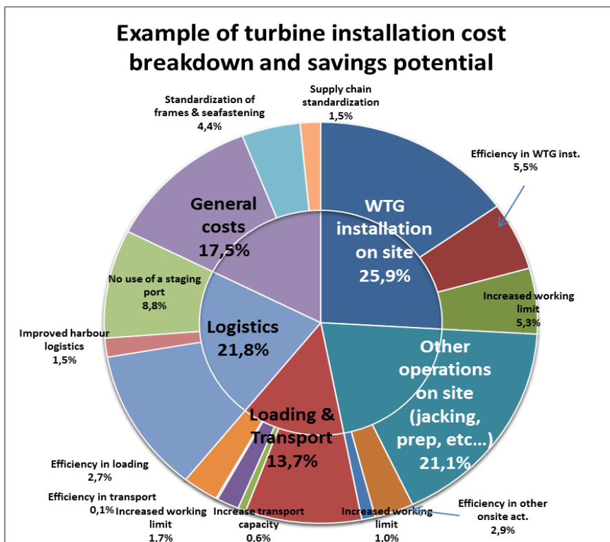
Figure 35: Turbine installation cost breakdown and savings potential. The inner circle reflects a high level breakdown whereas the outer circle shows the areas for cost reduction highlighted by the model. Source: Tractebel Engineering.
