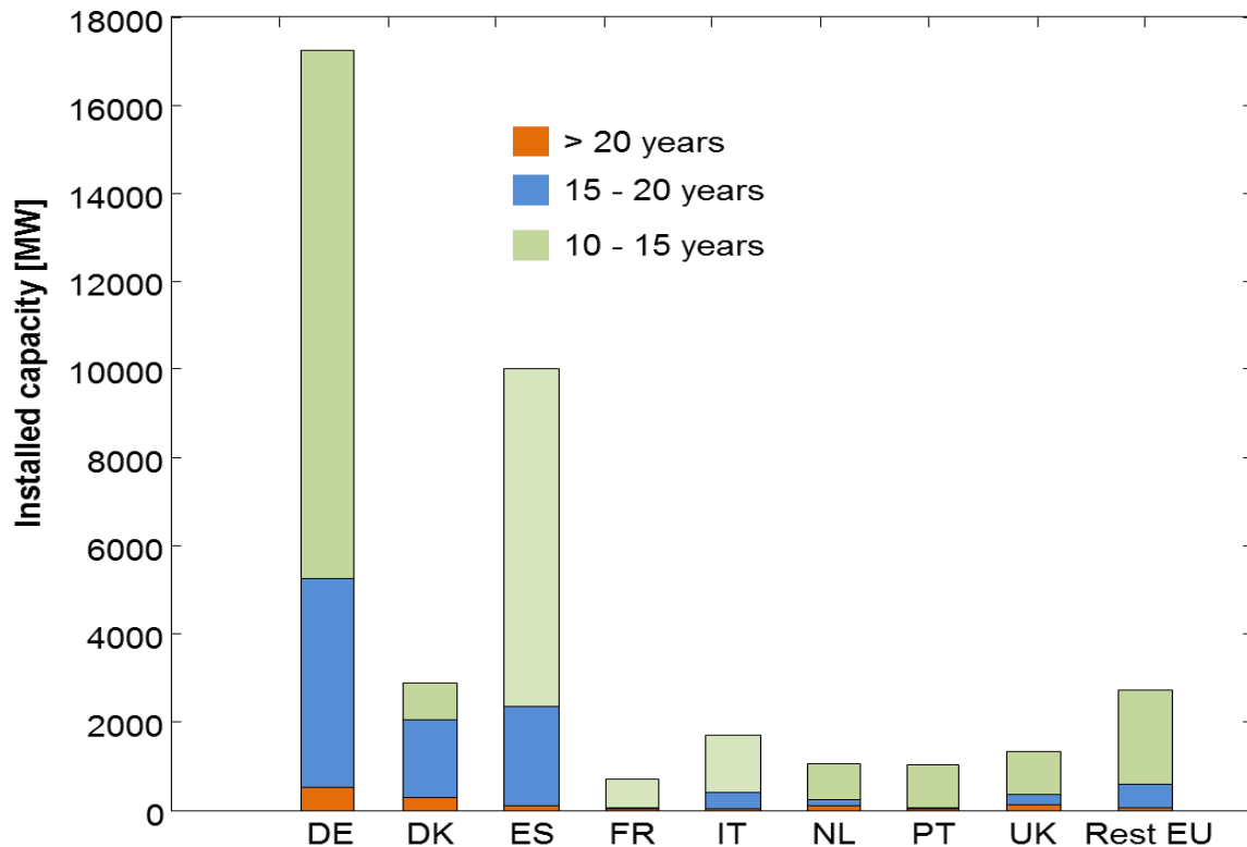
Figure 29: Wind installations older than ten years (at the end of 2013) in the EU Member States, showing the prospective repowering markets.
