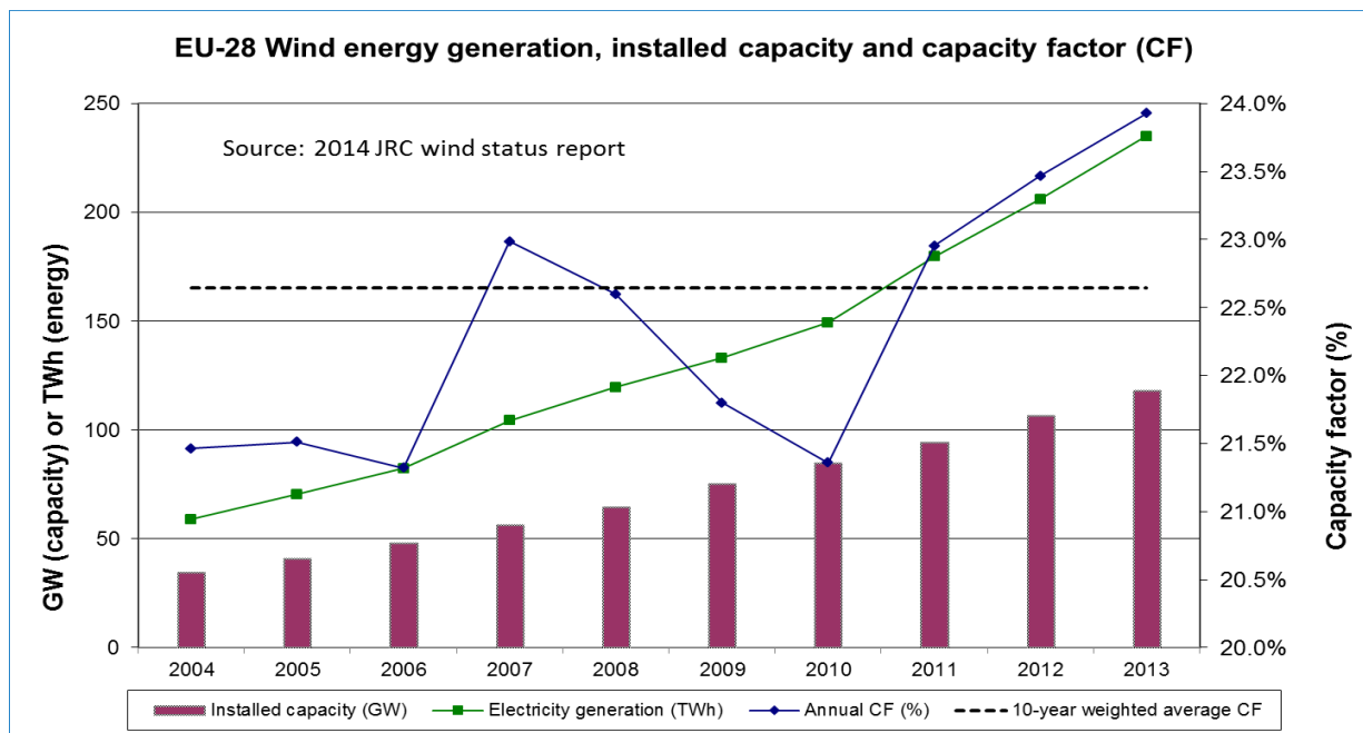
Figure 39: Set of production indicators for the EU per year — installed capacity, electricity generation and capacity factor. Source: JRC based on Eurostat and EWEA data.
