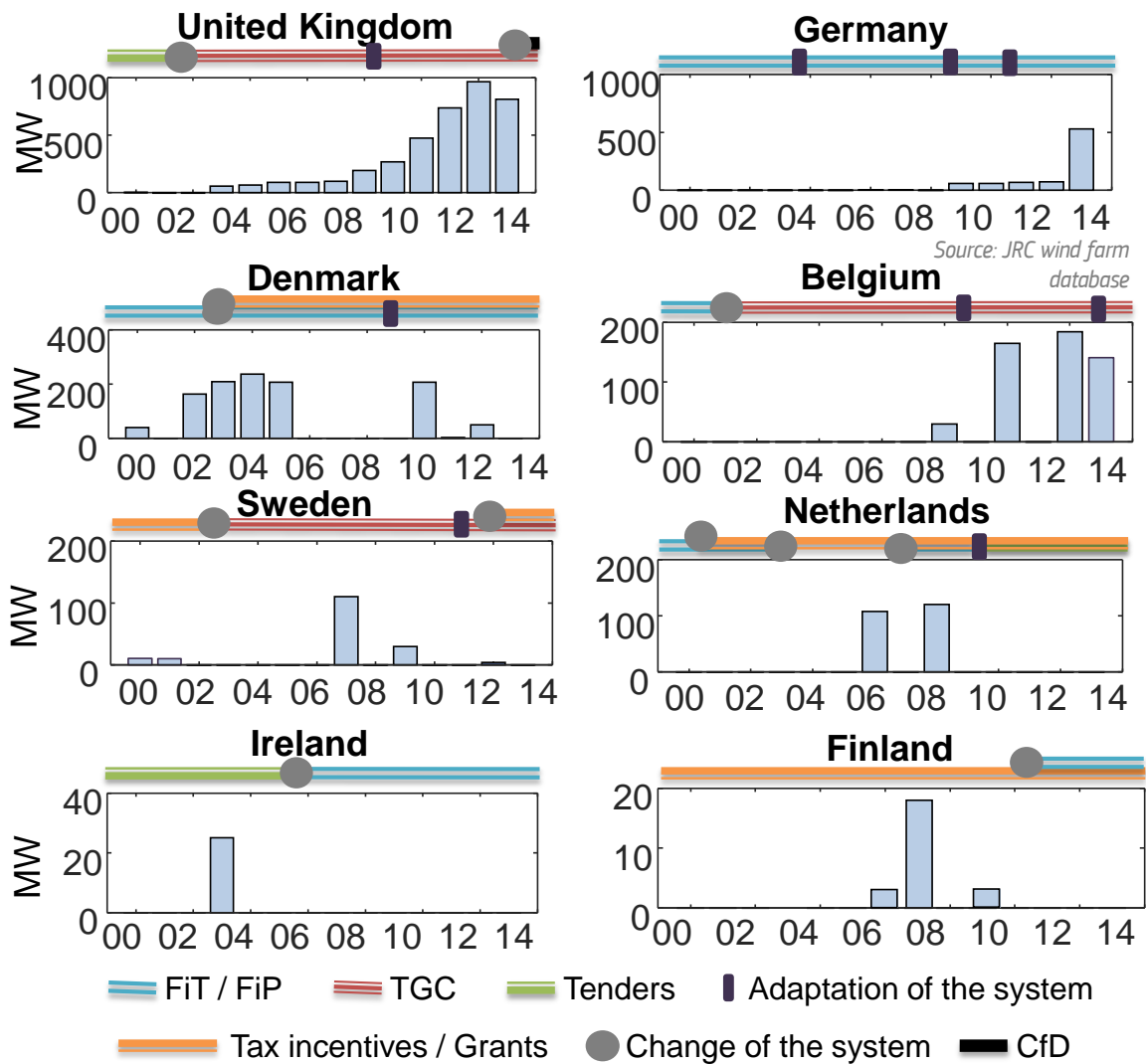
Figure 45: Annual deployment of offshore wind energy and evolution of support schemes in EU MSs countries.
