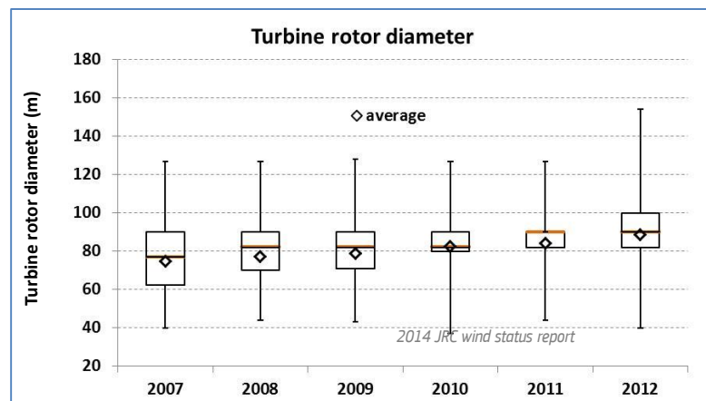
Figure 6: Boxplot representation of rotor diameters of onshore wind turbines installed each year in EU MS. (Source: JRC wind farm database).
