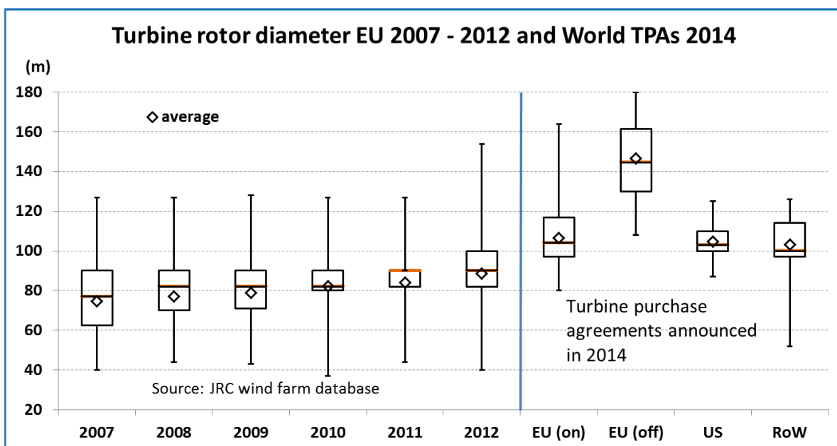
Figure 27: Rotor diameter in European turbines commissioned between 2007 and 2012, and in the TPAs disclosed in 2014. Source: JRC wind farm database.
