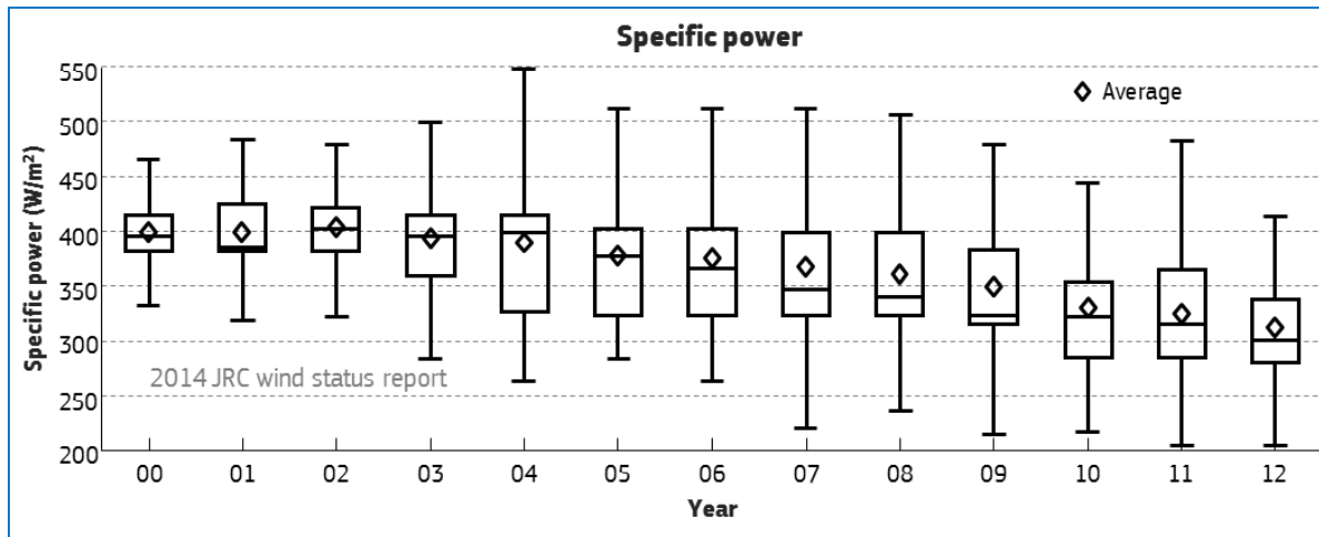
Figure 3: Boxplot representation of specific power ( W/m^2 ) for onshore wind turbines annually installed in the world. Bottom and top sides of each rectangle refers to the 25th and 75th percentiles. The horizontal line inside each rectangle represents the median and the lower and upper horizontal lines outside the rectangles are the minimum and maximum values. Source: JRC wind farm database.
