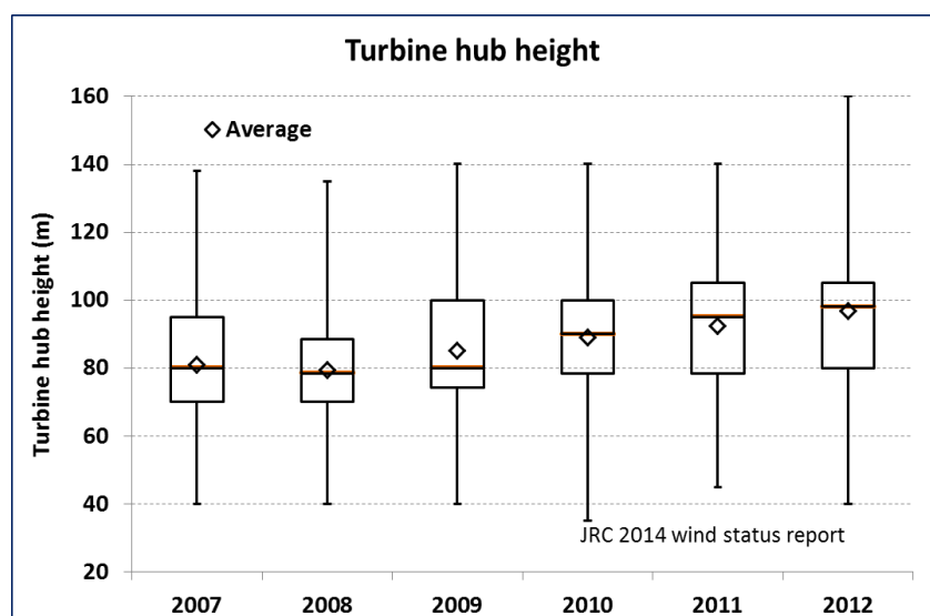
Figure 4: Boxplot representation of hub heights of onshore wind turbines installed each year in EU MS. Source: JRC wind farm database.
