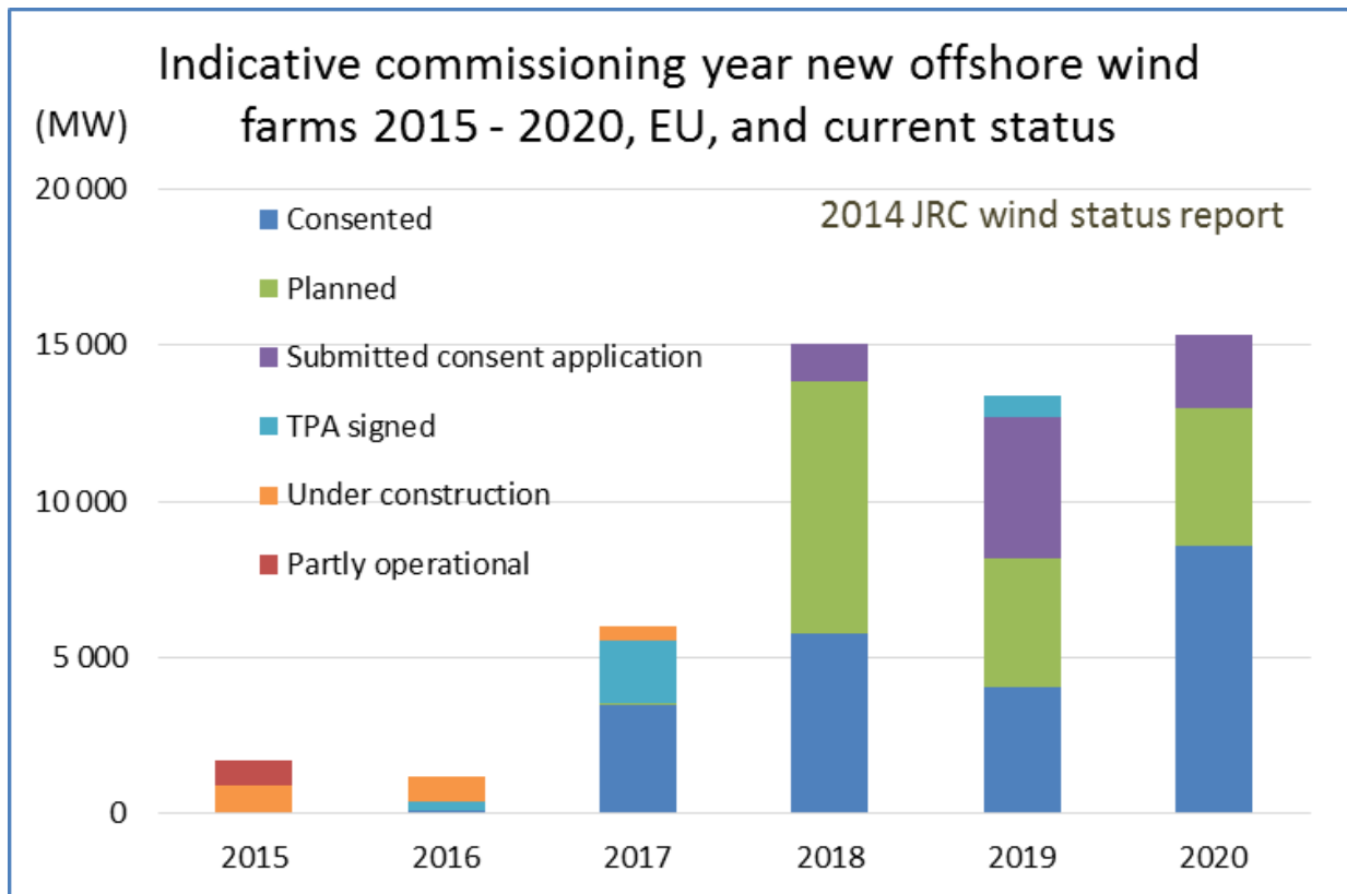
Figure 15: Status of the pipeline of offshore wind farms in the EU, in megawatts, according to the indicative commissioning year. TPA stands for turbine purchasing agreement. Source: JRC database.
