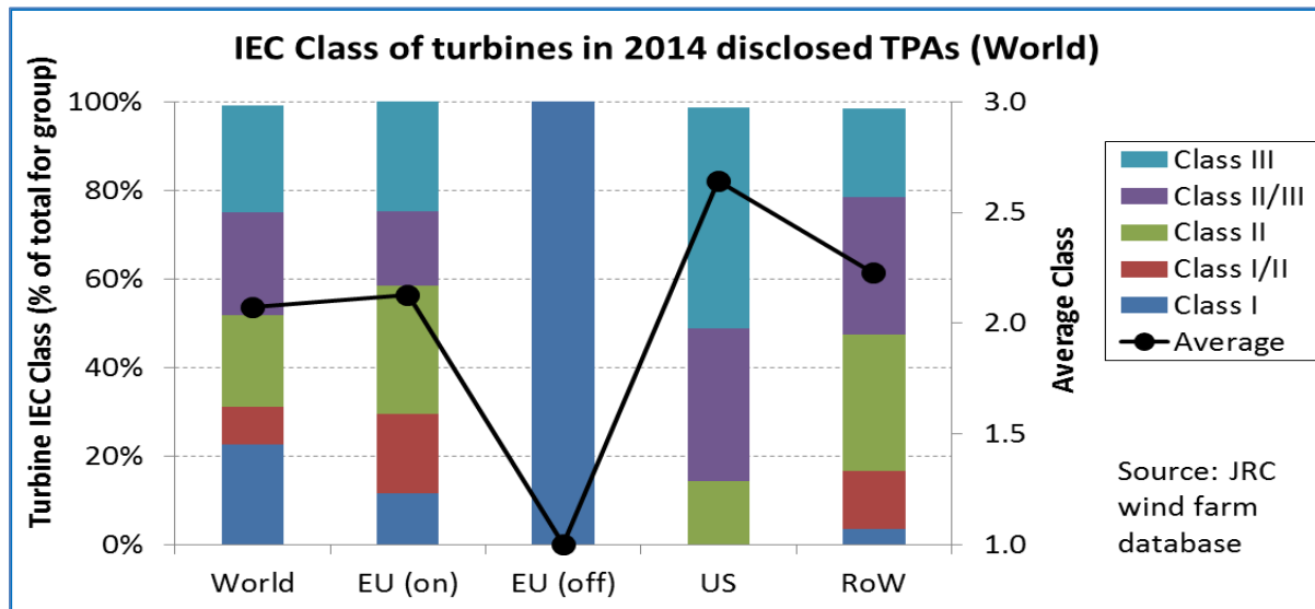
Figure 24: Breakdown of wind classes in the 2014 disclosed TPAs by group: US, EU onshore and offshore, rest of the world (RoW) and overall world figures.
