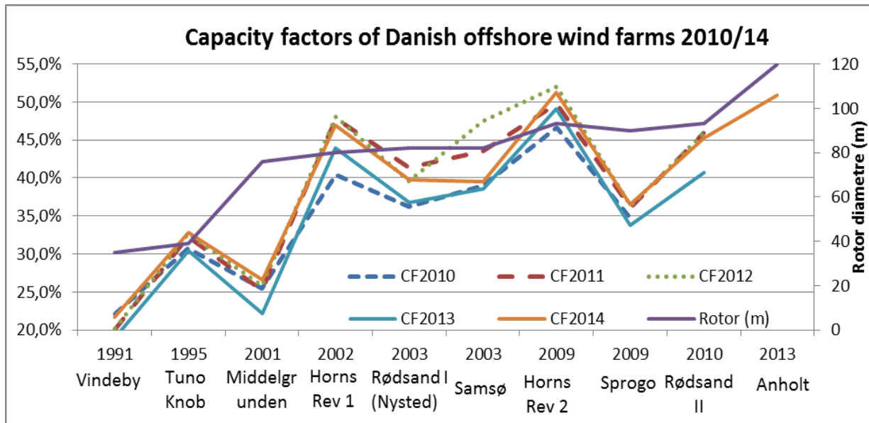
Figure 40: Capacity factors in Danish offshore wind farms related to the commissioning year. Source: JRC calculation from the Danish registry of wind turbines (Danish Energy Agency, 2015).
