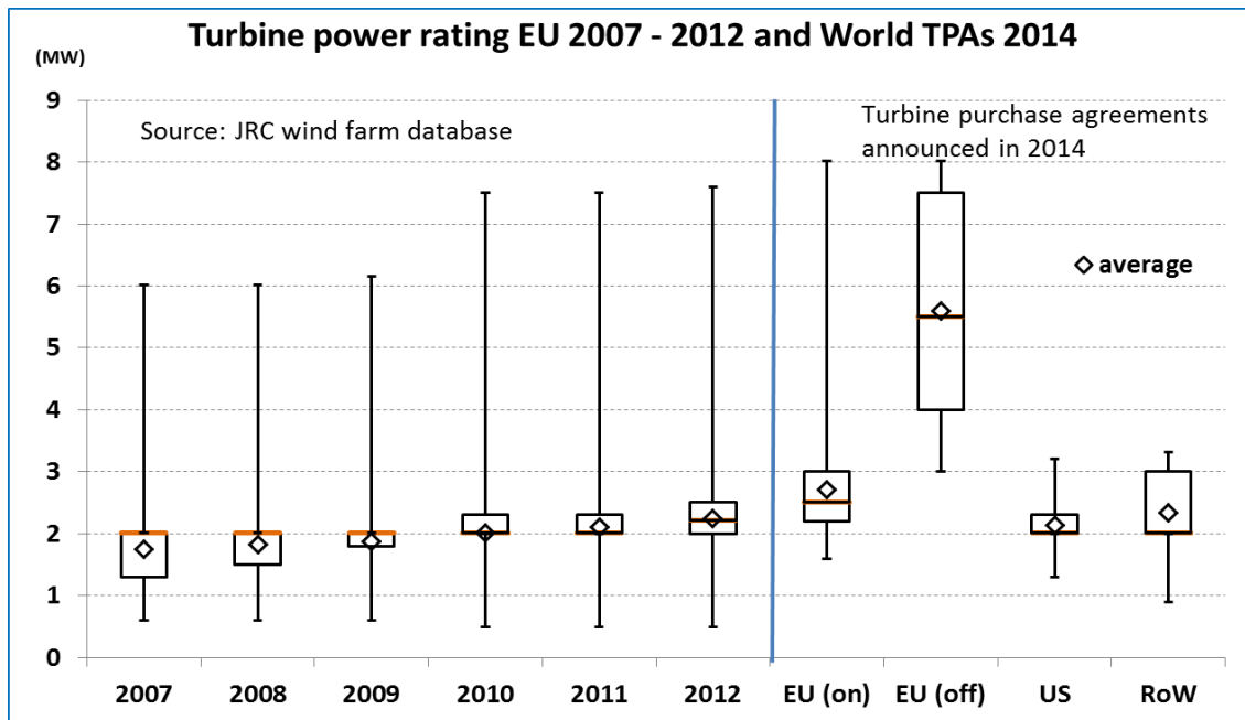
Figure 26: Turbine power rating in European onshore machines: evolution from 2007 to 2012 and comparison of data according to TPAs disclosed in 2014. Source: JRC database.
