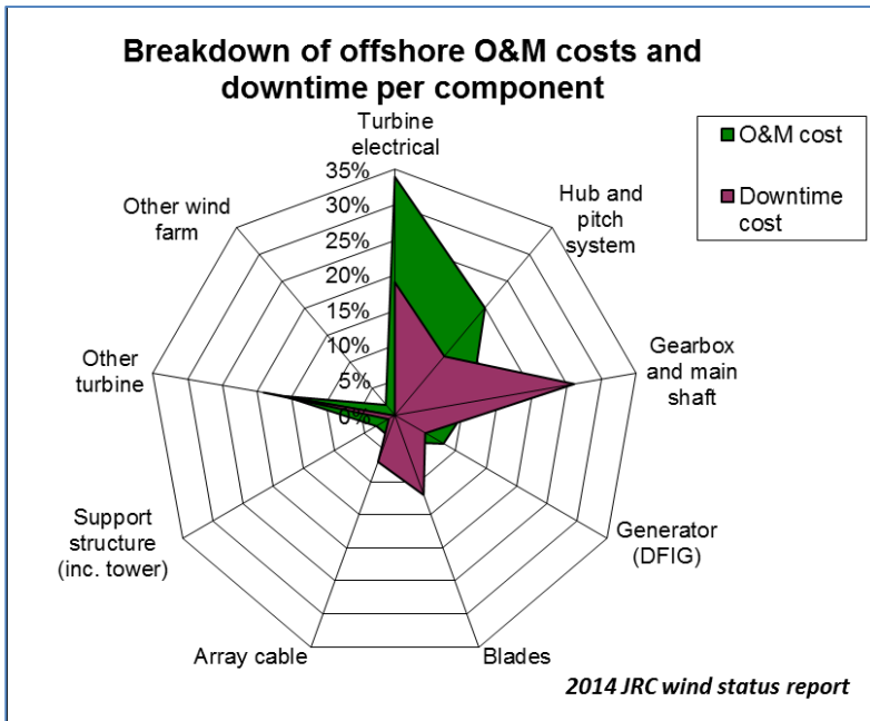
Figure 36: Breakdown of O&M costs, in percentage of monetary units, in an offshore wind farm. Source: JRC elaboration from (BVG, 2012).
