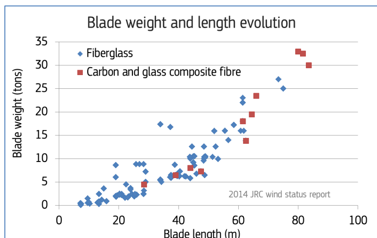
Figure 7: Blade weight relationship with length. (Source: BNEF and JRC wind turbines database).
