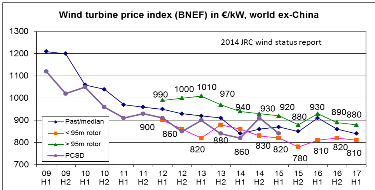
Figure 32: Evolution of wind turbine prices based on the year of delivery (past/median, less or more than 95 metres rotor) and per year of contract signature (PCSD), except China. Source: BNEF (2015c).
