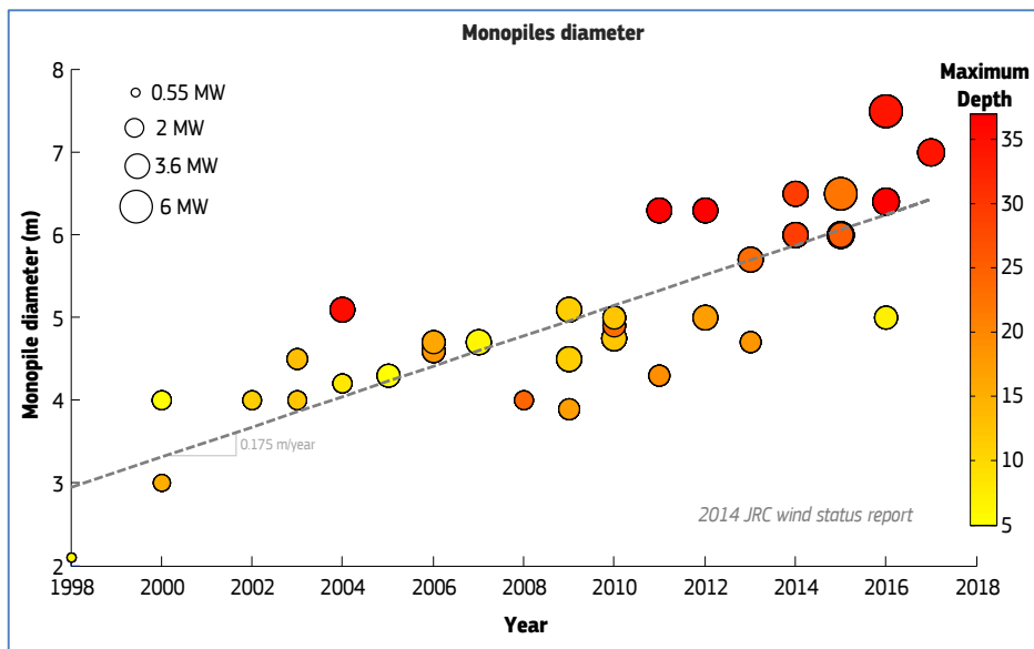
Figure 11: Evolution of monopiles diameter (installed and planned). Circle size relates to wind turbine rated power and colour to maximum seabed depth at the wind farm location.
