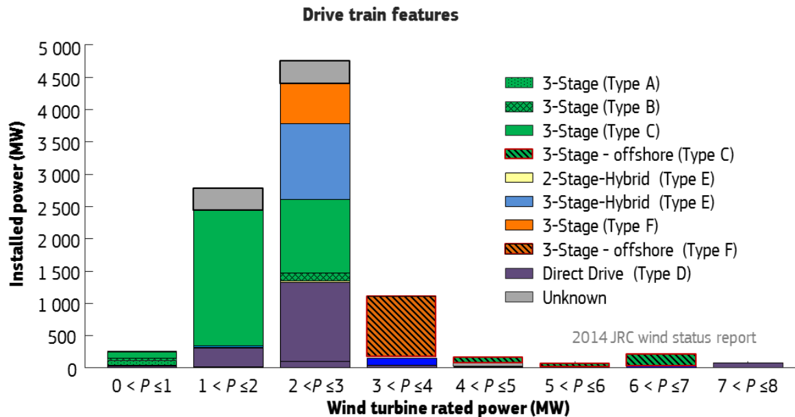
Figure 9: Drive train features classified according to wind turbine rated power. Data corresponding to installations in EU MS during 2012. Source: JRC Database.
