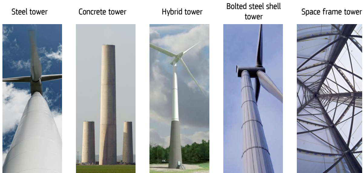
Figure 5: Different kinds of towers. Courtesy: Siemens, Acciona, GRI Renewable Industries and General Electric.
