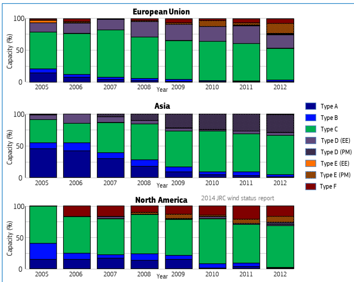
Figure 8: Evolution of the share of installed capacity by wind turbine configuration (Source: JRC Database). PM: permanent magnet, EE: electromagnetic excitation.
