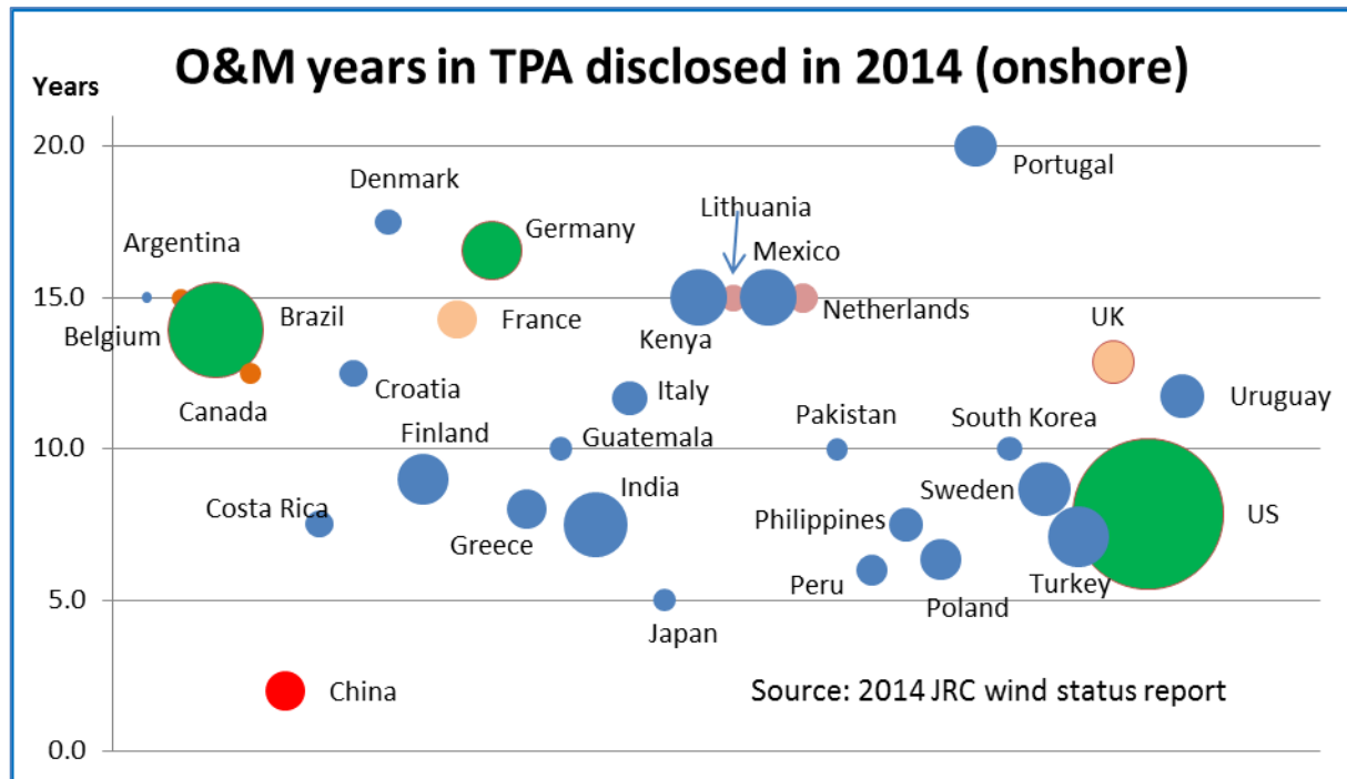
Figure 37: Length of O&M contracts included as part of turbine purchase agreements. The thickness of the bubbles represents the country volume in MW, whereas the horizontal axis does not have any unit. Source: JRC.
