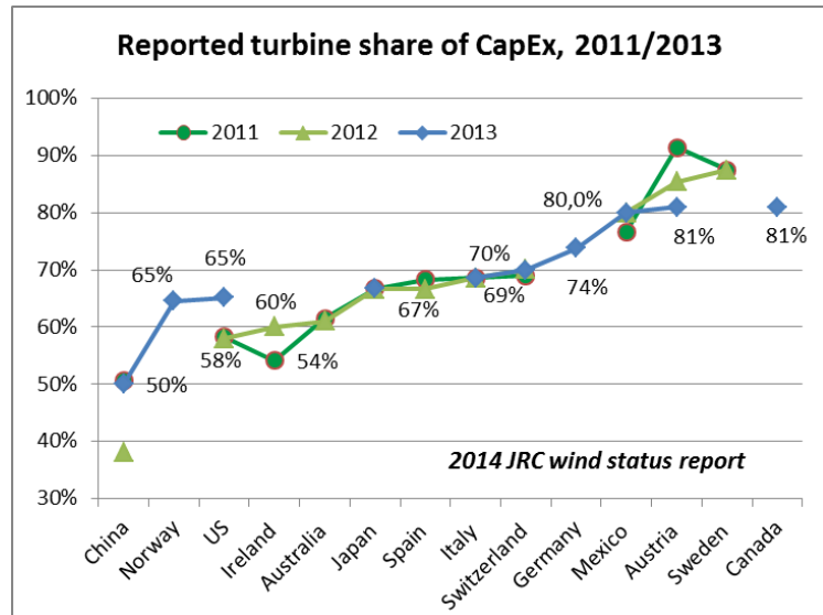
Figure 33: Turbine share of CapEx in onshore projects, 2011, 2012 and 2013. Source: JRC elaboration with data from IEAWind (2012, 2013, 2014).
