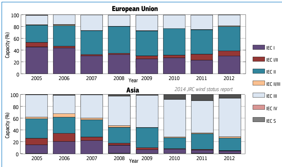
Figure 2: Evolution of the share of onshore installed capacity by wind classes (Source: JRC Database). See Table 1 for a definition of wind classes according to IEC 61400.
