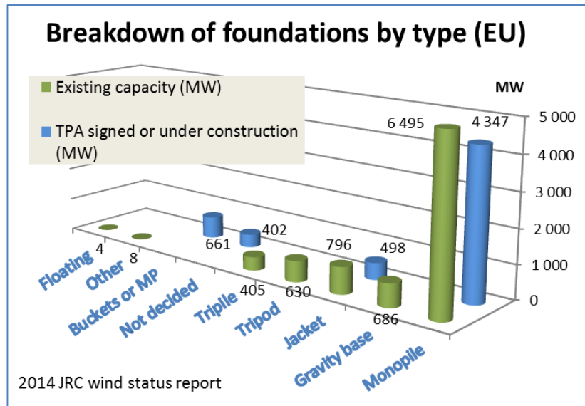
Figure 10: Split of foundations by type, both for existing wind farms and for wind farms under construction (early 2015). Source: JRC database.
