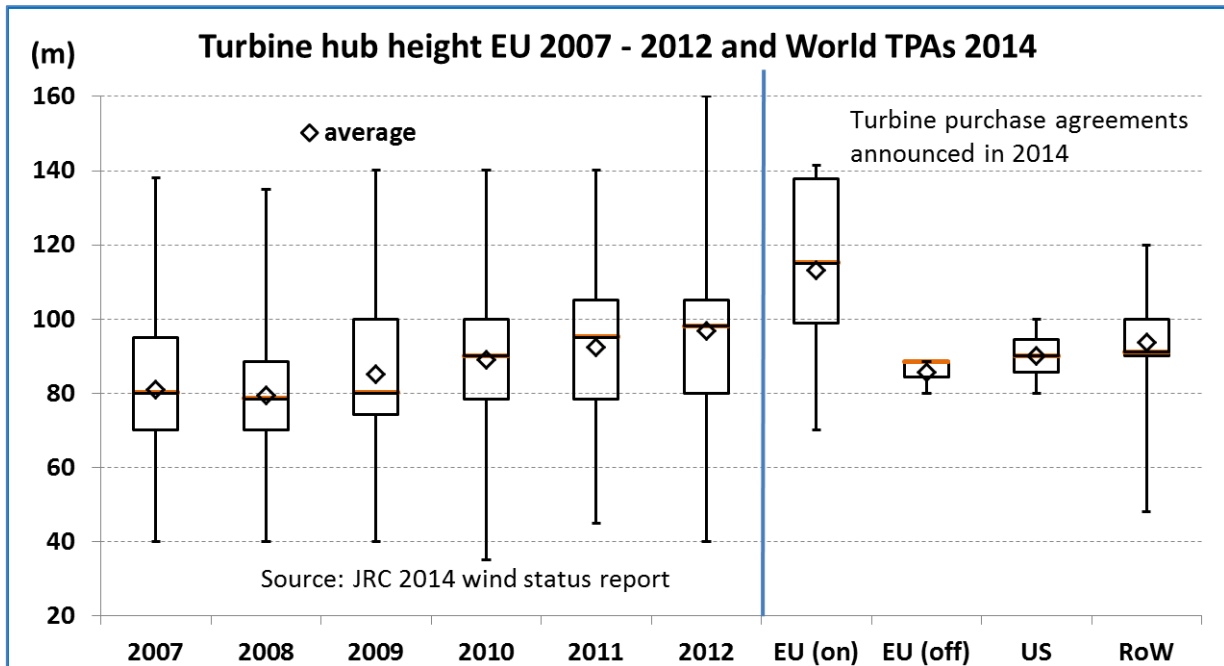
Figure 28: Plot of turbine hub height in turbines installed in the EU during 2007–12, and in the TPAs disclosed in 2014
