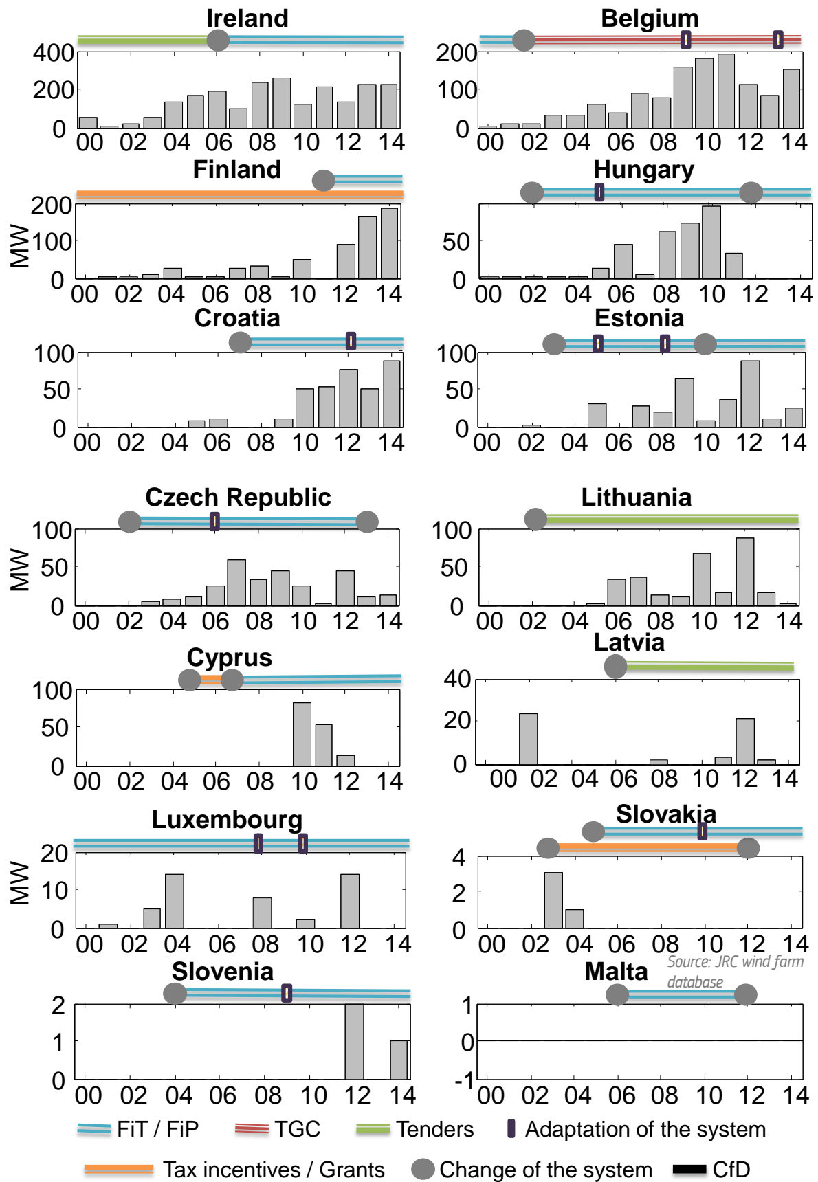
Figure 44: Annual deployment of onshore wind energy and evolution of support schemes in EU MSs countries.
