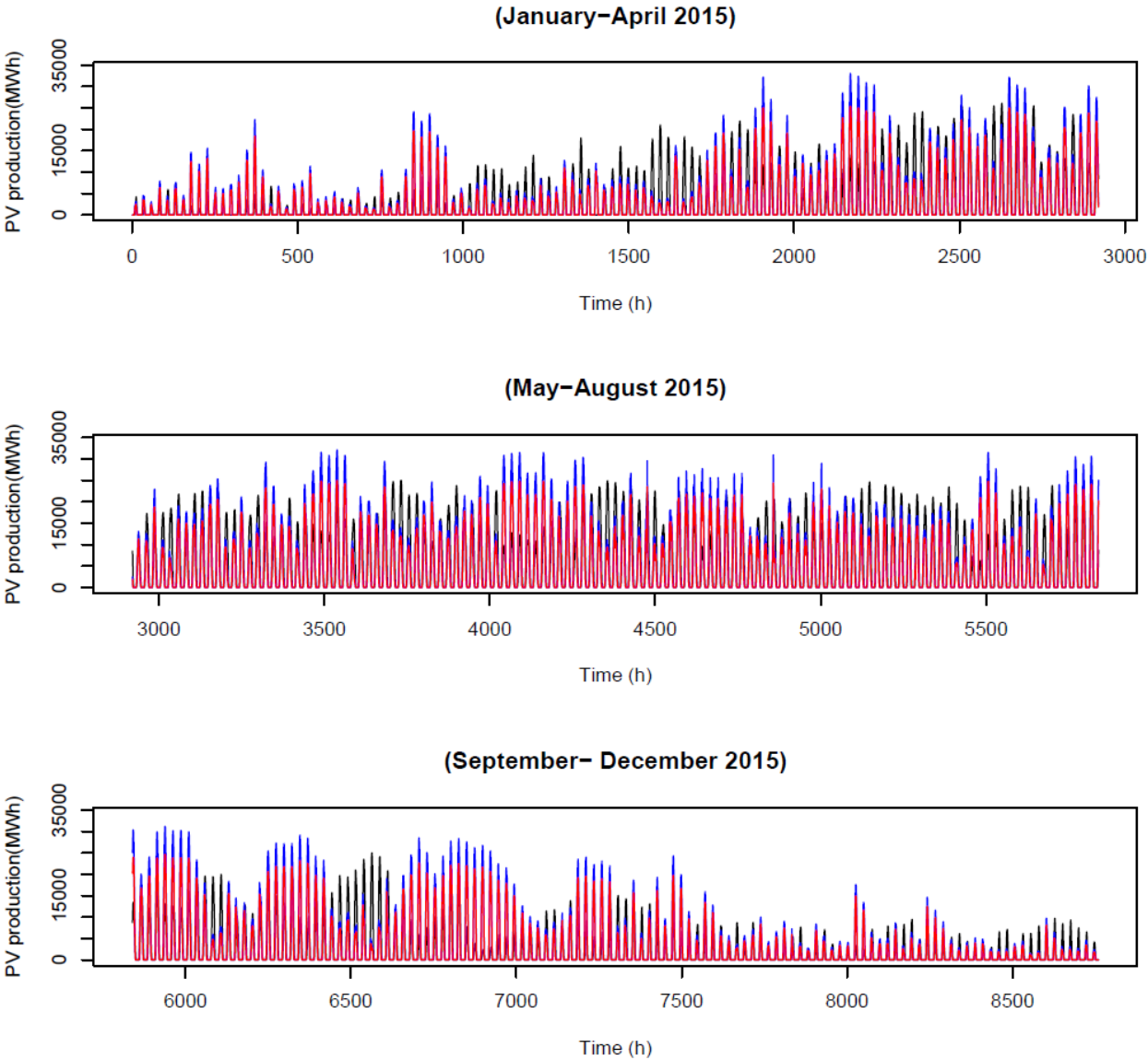
Figure 6. PVGIS-derived (blue), PVGIS-corrected (red) and TSO (black) power generation hourly time series for Germany 2015
