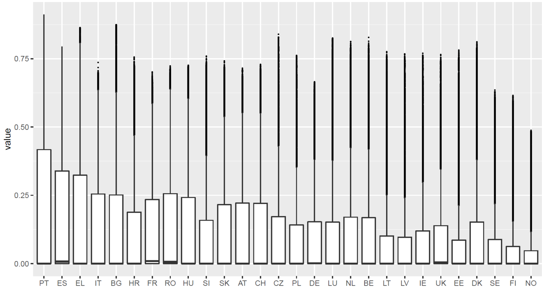
Figure 9. Boxplot of the capacity factors by country for the 30-year period (1986-2015)
